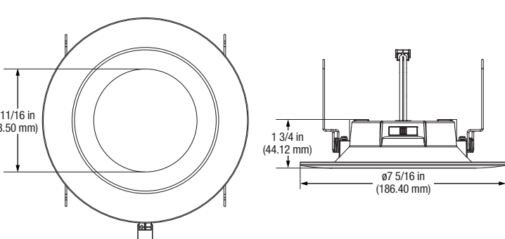
6" SMOOTH
