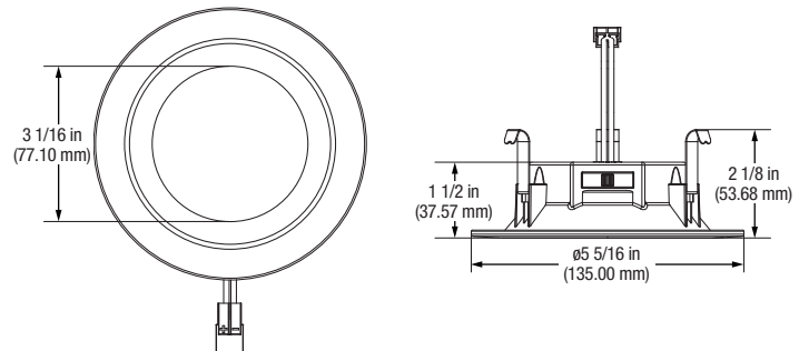
6" SMOOTH
