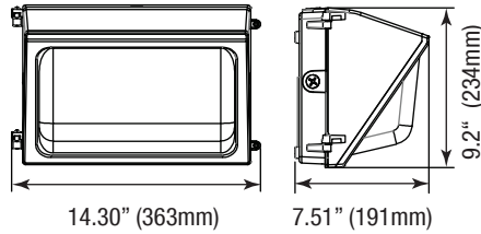
38W 6.79-lbs
