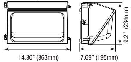
80W 8.07-lbs
