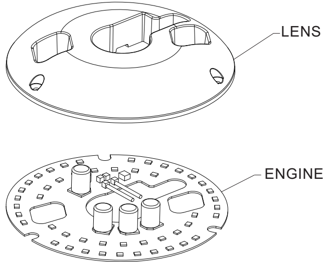
Exploded View
