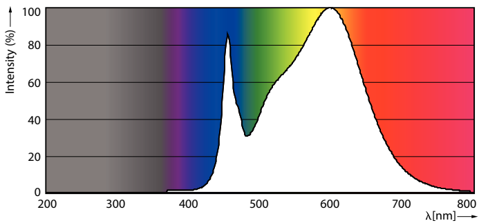
LEDTube_10T8_COR_48-835_IF15_G 10_1-POC
