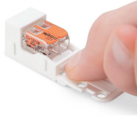
Removing a connector from the mounting carrier.
