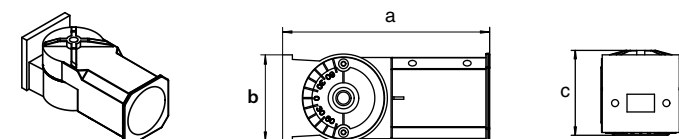
Slip Fitter
