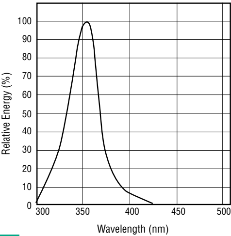
Blacklight Lamp (BL) 352nm
