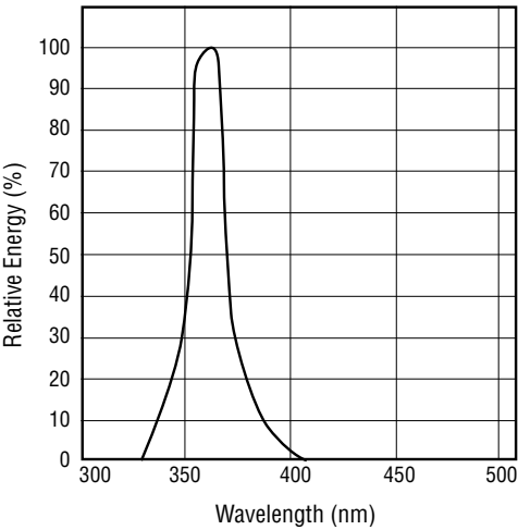
Blacklight Blue Lamp (BLB) 368nm
