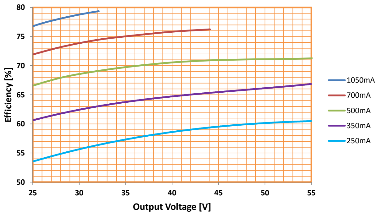
Efficiency @ Step-Dim
