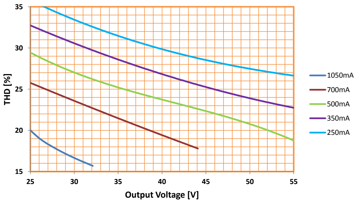
THD @ Step-Dim
