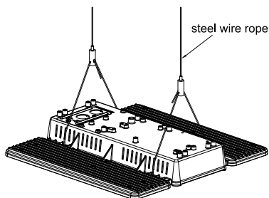
Suspended Mounting
