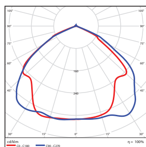
LED7PL- Horizontal
