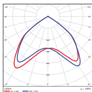
LED7PL- Vertical
