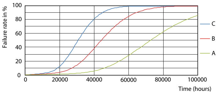
LEDtube_70K_FailureRate-LED
