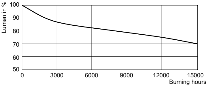
CDM-Rm 20W Lumen Maintenance /830 VBU
