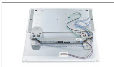
Step 1: EvoKit with Xitanium SR is shipped with a plate covering the sensor hole. There are two wires secured to the back of the plate.
