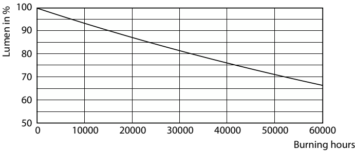
Lumen Maintenance Diagram - 36-27-18CC/LED/3PW/3CCT/E26 BB 6/1
