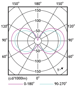
Light Distribution Diagram - 27-18-12CC/LED/3PW/3CCT/E26 BB 6/1
