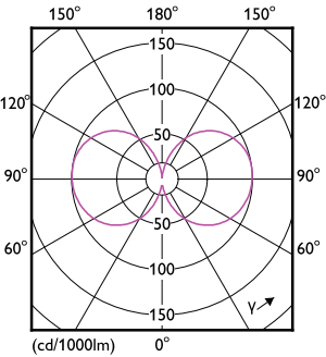
Light Distribution Diagram - 54GC/LED/830 EX39 BB 6/1
