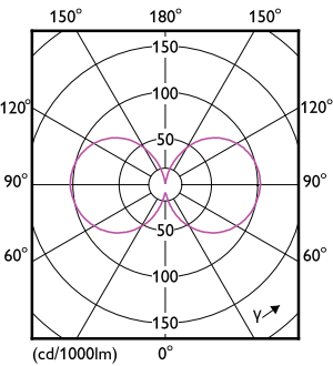
Light Distribution Diagram - 34GC/LED/840 EX39 BB 6/1
