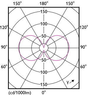
Light Distribution Diagram - 15GC/LED/830/ND E26 BB 6/1
