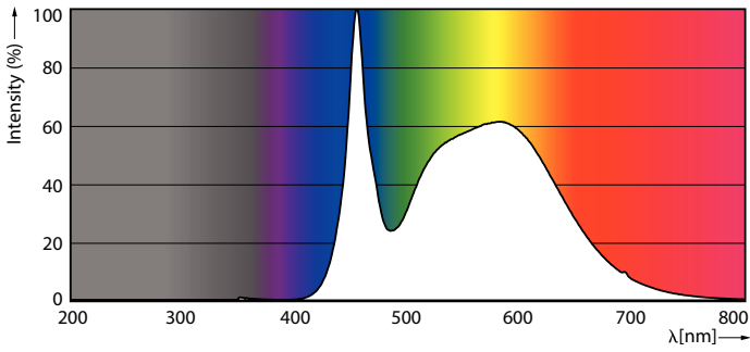
Spectral Power Distribution Colour - 15GC/LED/830/ND E26 BB 6/1
