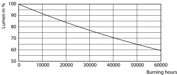
Lumen Maintenance Diagram - 10PAR30L/EXPERTCOLOR/ F40/940/P/D/T/JA8
