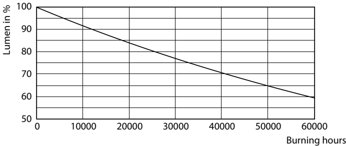
Lumen Maintenance Diagram - 10PAR30L/EXPERTCOLOR/ F25/940/P/D/T/JA8
