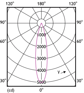
Light Distribution Diagram - 10PAR30S/EXPERTCOLOR RETAIL/S10/930/D
