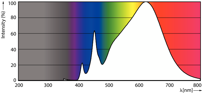
Spectral Power Distribution Colour - 10PAR30S/EXPERTCOLOR RETAIL/S10/930/D
