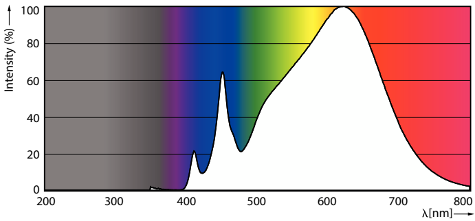
Spectral Power Distribution Colour - 10PAR30L/EXPERTCOLOR RETAIL/F40/930/D
