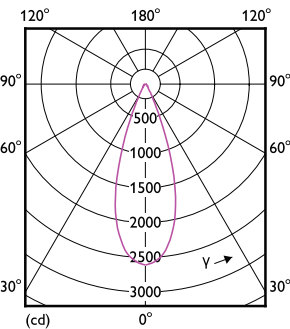
Light Distribution Diagram - 10PAR30L/EXPERTCOLOR RETAIL/F40/930/D
