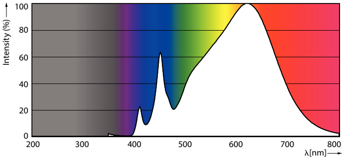
Spectral Power Distribution Colour - 10PAR30L/EXPERTCOLOR RETAIL/S10/930/D
