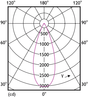
Light Distribution Diagram - 14PAR38/EXPERTCOLOR/ F40/927/P/D/T20/JA8
