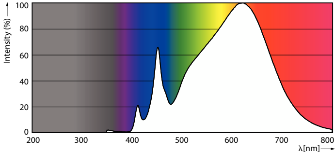
Spectral Power Distribution Colour - 14PAR38/EXPERTCOLOR RETAIL/ F40/930/P/D
