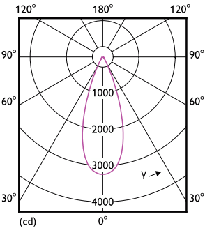
Light Distribution Diagram - 14PAR38/EXPERTCOLOR RETAIL/ F40/930/P/D
