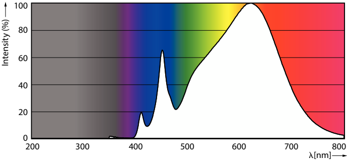
Spectral Power Distribution Colour - 14PAR38/EXPERTCOLOR RETAIL/F25/930/P/D
