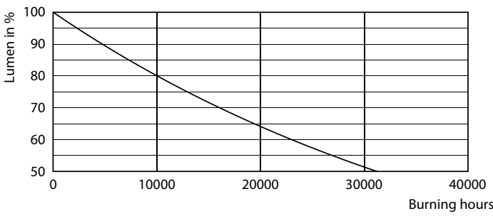
Lumen Maintenance Diagram - CorePro LEDbulb ND 12.5-100W A60 E27 940
