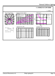
General uniform lighting - 10A19/CNG/850/FR/P/E26/ND 4/1CT
