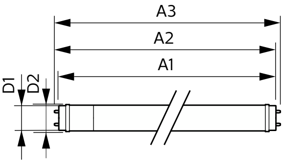
11.5T8/COR/48-840/IF21/G/DIM 25/1
