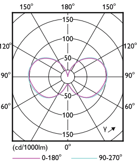
LEDTForce LS DLC 63W Corncob EX39-LDD
