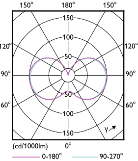
LEDTForce LS 80W Corncob EX39-LDD
