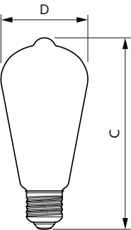
5.5ST19/VIN/950/E26/CL/G/SP D 4/1PF T20
