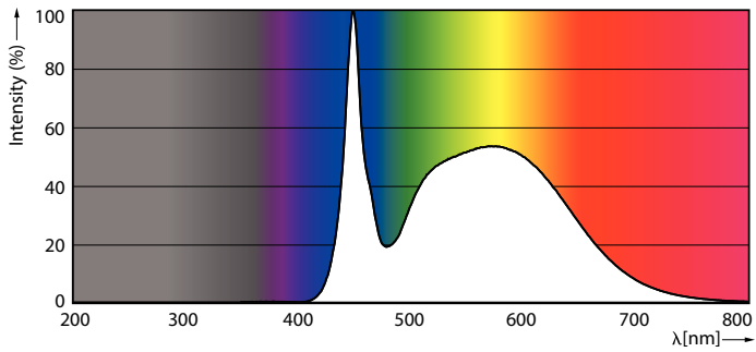
LEDtube COR 11W G13 1700lm 850
