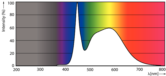
LEDTForce 60W WallPack EX39 850
