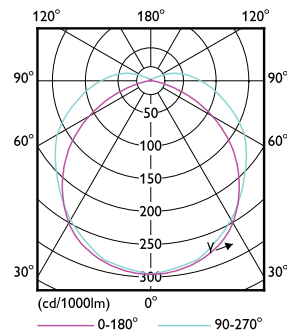
LEDTForce WallPack
