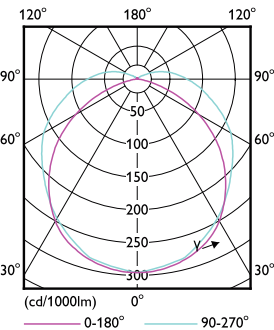
LEDTForce WallPack
