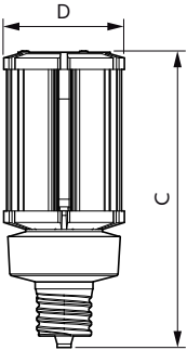
Corn lamp LED Gen2 36W EX39 830 CL
