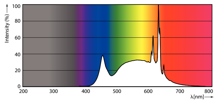
LEDbulb 16W A19 E26 940 FR
