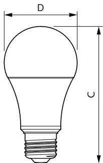
Bulb A19 120V 16-100W 1600lm 4000K E26 D
