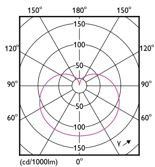
LEDbulb A19 16W E26 1600lm 940 FR
