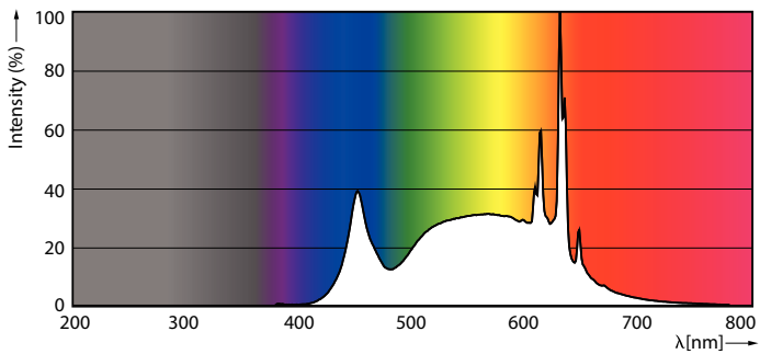
LEDbulb 12,2W A19 E26 940 FR
