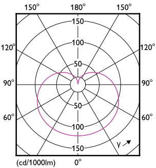
LEDbulb A19 12,2W E26 1100lm 930 FR
