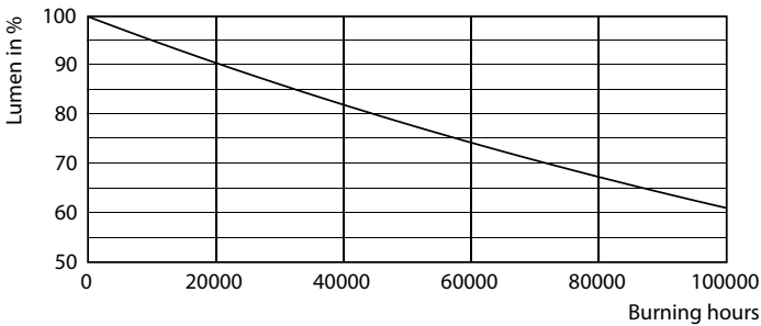
LEDtube_70K-LMP
