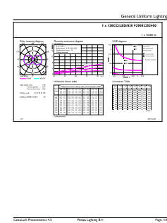
Corn lamp LED 120W EX39 830 CL
