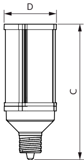
Corn lamp LED 54W EX39 830 CL
