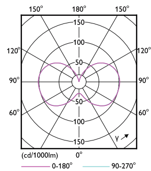
Corn lamp LED 54W EX39 830 CL
