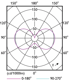
Corn lamp LED 36W E26 830 CL
