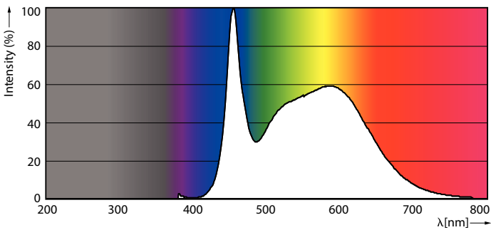
Corn lamp LED 36W E26 850 CL
