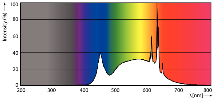
40W E26 A19 940 Frosted
