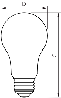
Bulb A19 120V 5-40W 450lm 4000K E26 D
