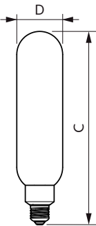
Bulb T65 120V 8-40W 450lm 2000K E26 D
