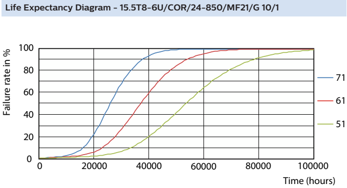
Life Expectancy Diagram - 15.5T8-6U/COR/24-850/MF21/G 10/1
