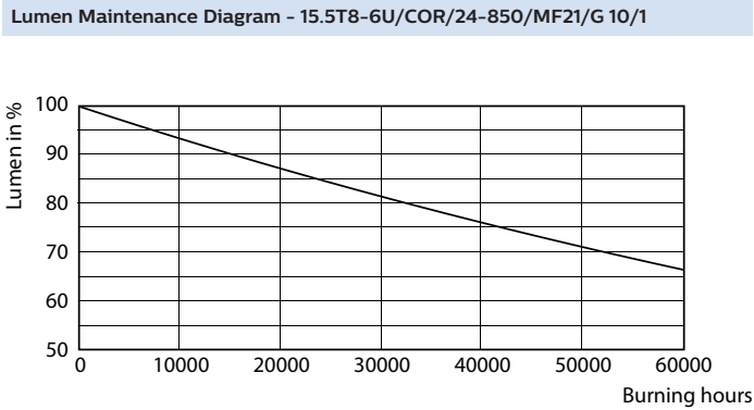
Lumen Maintenance Diagram - 15.5T8-6U/COR/24-850/MF21/G 10/1
