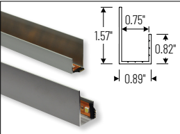
4' J-Style Channel
