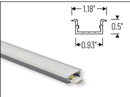
4' Shallow Recessed Channel
