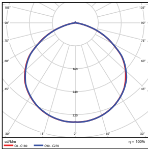
HBR135 (134 Watt) DLC Premium
