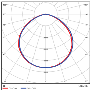
HBR90 (90 Watt) DLC Premium
