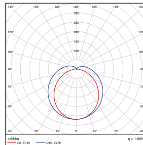
FXCSL (4')- 35 Watt DLC Premium
