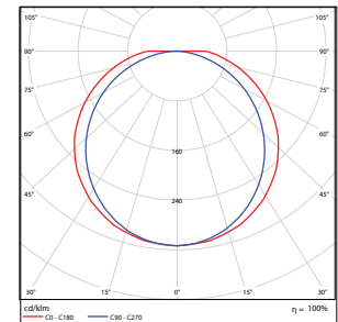
FXCSL (8')- 42 Watt DLC Premium
