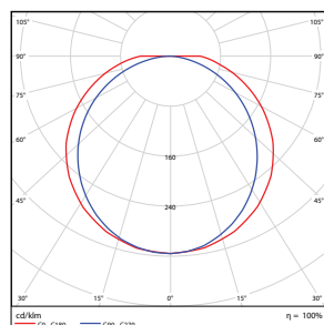
FXCSL (8')- 56 Watt DLC Premium
